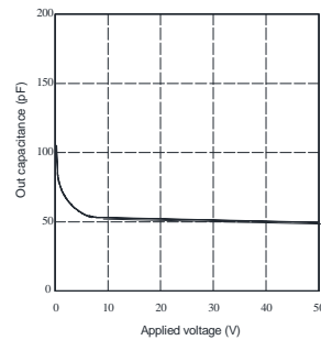
Applied voltage Vs. output capacitance characteristics
