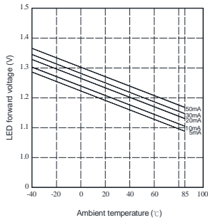
LED forward voltage Vs. Ambient temperature
