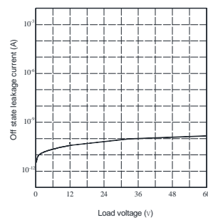
Off state leakage current Vs. Load voltage characteristics
