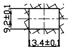
Panel Installation Thickness 1 ~ 4mm
