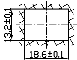
Panel Installation Thickness 0.8 ~ 2mm
