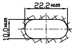
Panel Installation Thickness 1 ~ 4mm
