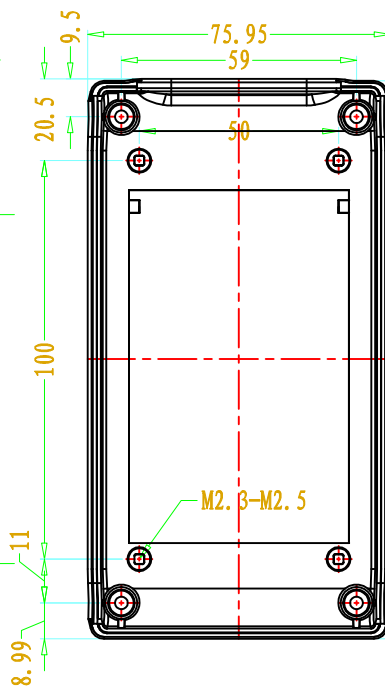
SEC B-B
