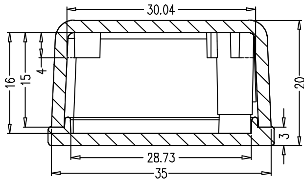
SEC B-B
