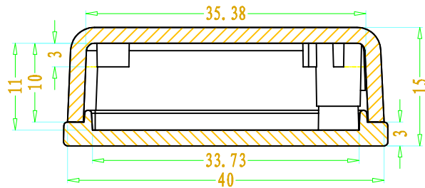
SEC B-B
