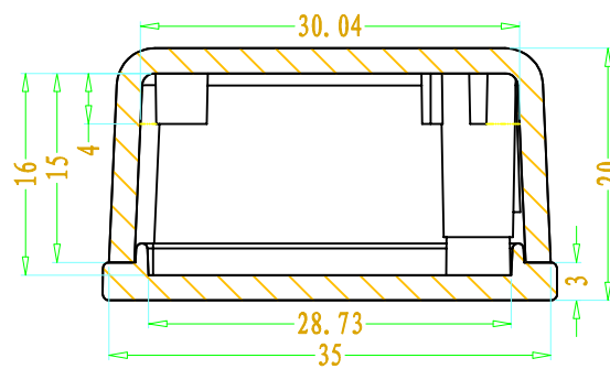
SEC B-B
