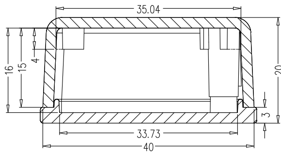
SEC B-B
