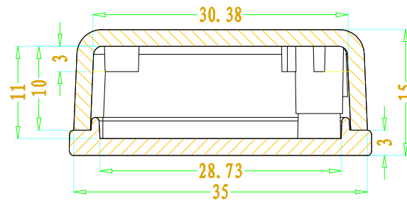
SEC B-B
