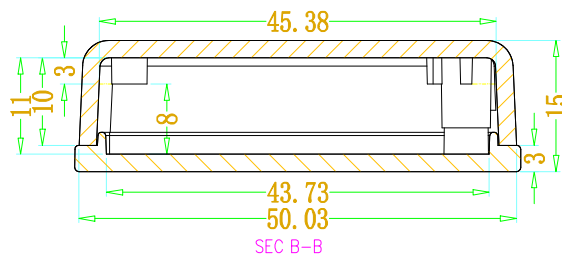
SEC B-B
