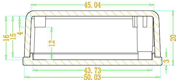
SEC B-B
