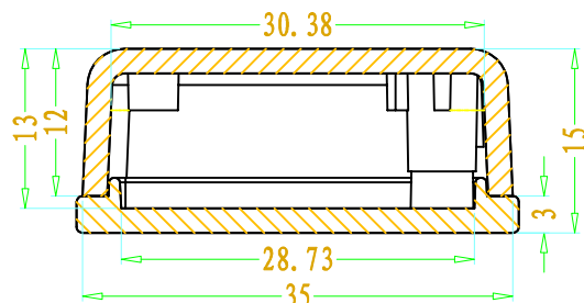
SEC B-B
