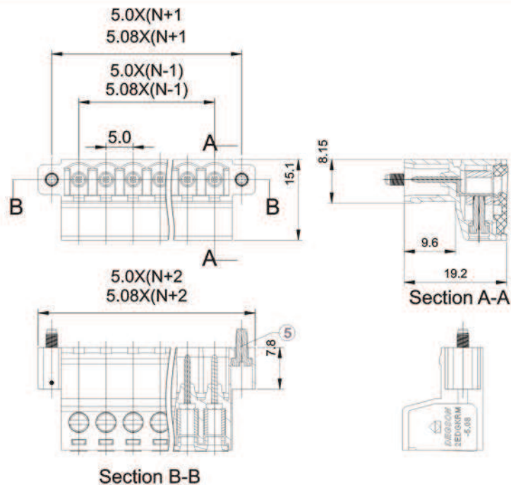
2EDGKRM-5.0 2EDGKRM-5.08
