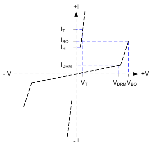
V - I Characteristics
