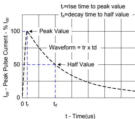
t_r \times t_d Pulse Waveform
