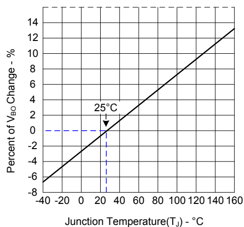
Normalized V_{BO} Change versus Junction Temperature
