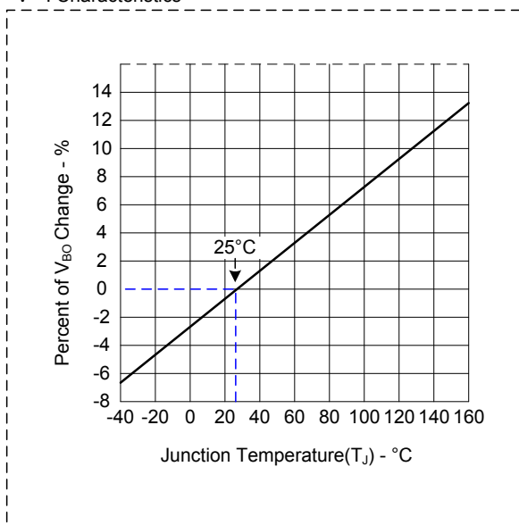
Normalized V_{BO} Change versus Junction Temperature
