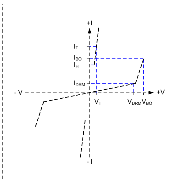
V - I Characteristics
