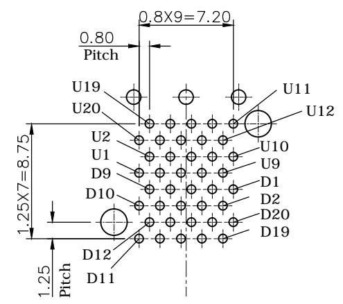
Detail D Scale 2.5/1
