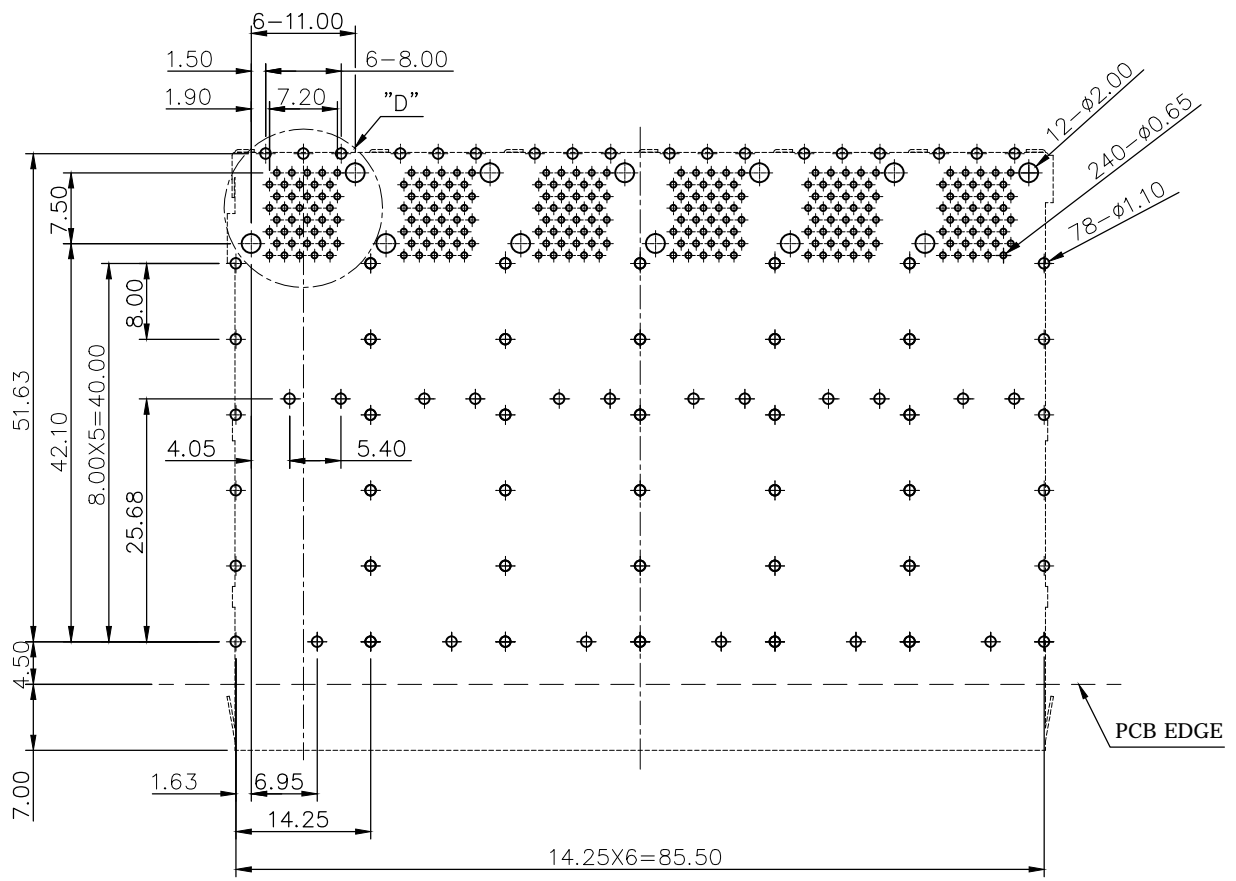
RECOMMENDED LAYOUT (TOP VIEW) GENERAL TOLERANCE: ±0.05mm
