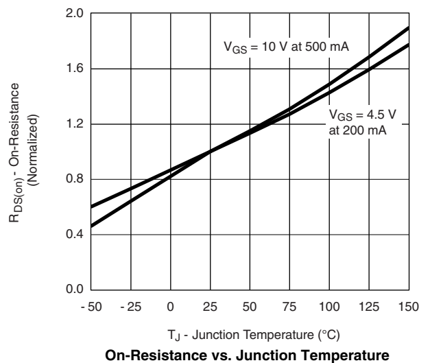
V_{GS} = 10 V at 500 mA V_{GS} = 4.5 V at 200 mA On-Resistance vs. Junction Temperature
