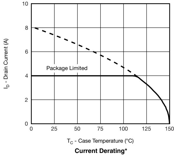
Current Derating*
