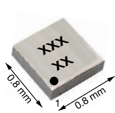
Backside View
