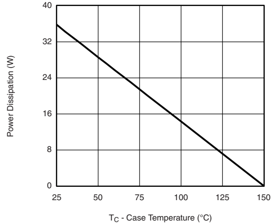
Power Derating
