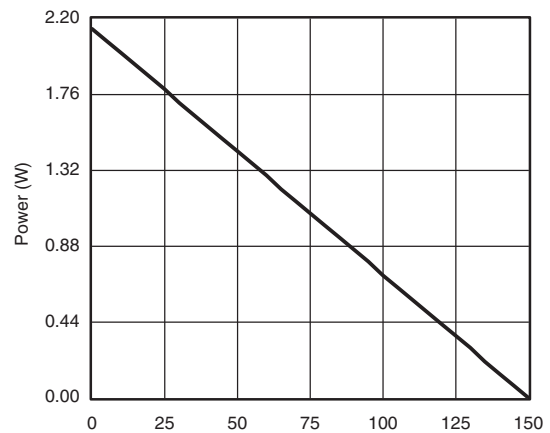
Power, Junction-to-Ambient
