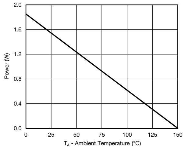
Power, Junction-to-Ambient
