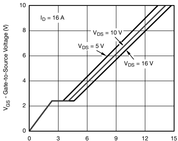
Gate Charge
