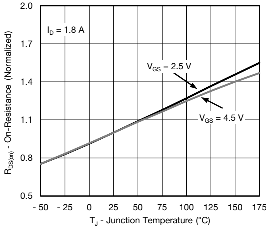
On-Resistance vs. Junction Temperature (1.8 A)
