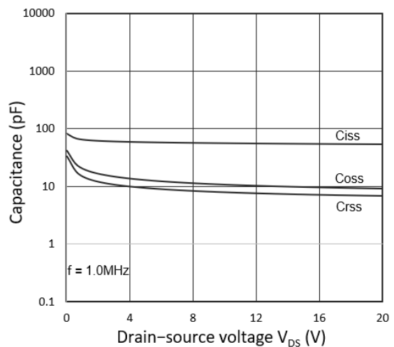
Figure 6. Capacitance Characteristics
