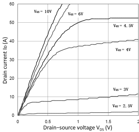
Figure 1. Output Characteristics
