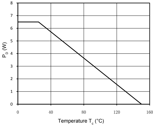
Figure 9. Power Dissipation
