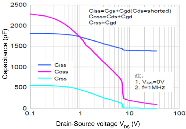
Figure 7. Capacitance Characteristics
