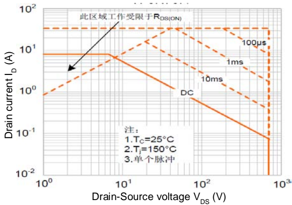
Figure 9. Maximum Safe Operating Area (WML07N65DM)
