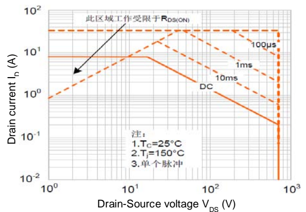
Figure 10. Maximum Safe Operating Area (WMK/M/N07N65DM)
