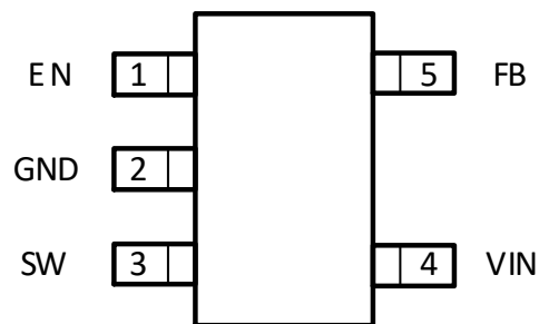
SOT23-5(Top View)
